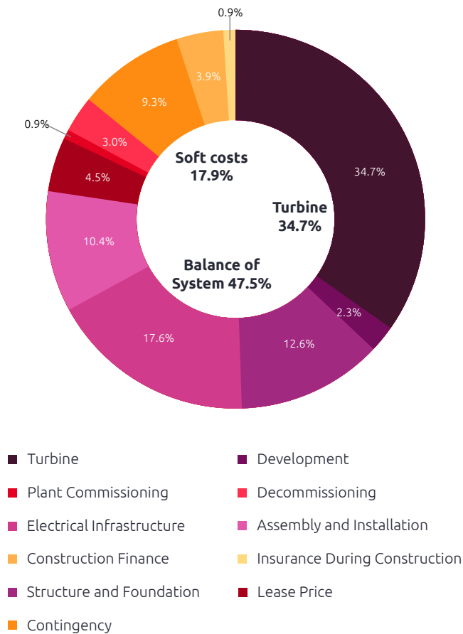
FIGURE 4 CAPEX for typical fixed-bottom offshore wind farm, 2020
