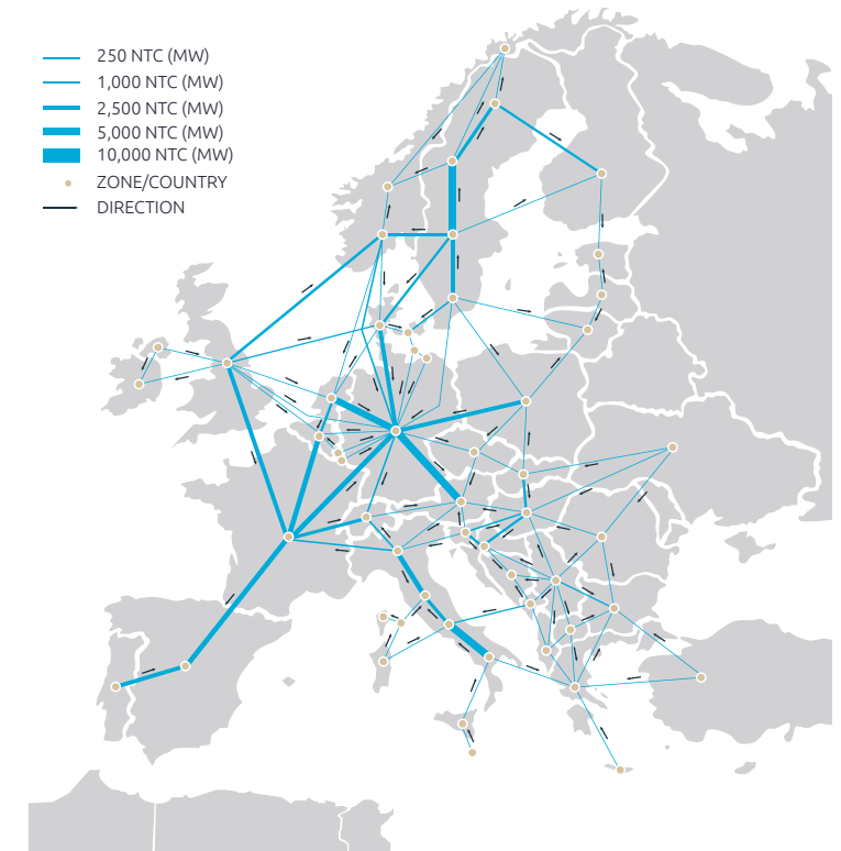
Standard Net Transfer Capacity model for 2030
